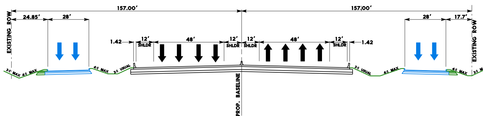
PROPOSED TYPICAL SECTION SECTION C-C
